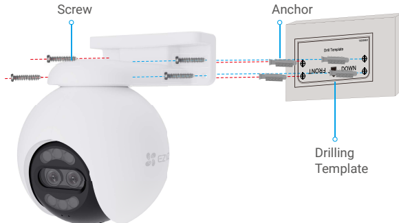
Fig. 2 Wall Mount
